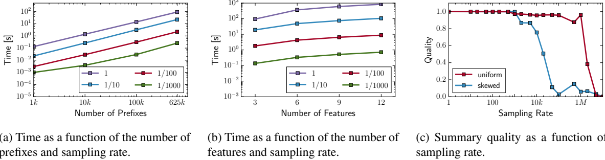
Figure 4: Net2Text scales—both in the size of the forwarding state (sub-second, even for 625k prefixes) (a) and the number of features (sub-second, even for 12 features) (b)—while sampling affects the summary quality marginally (c).
