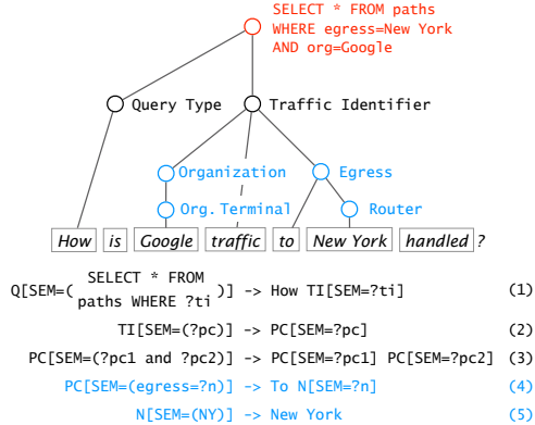
Figure 3: A parse tree and rules in the network grammar.
