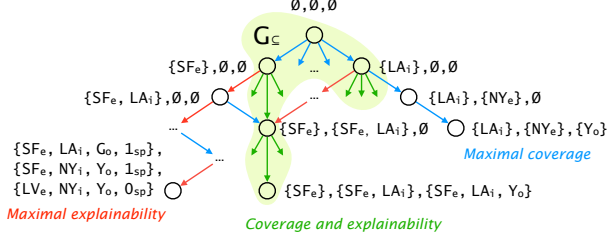
Figure 2: Part of the search space for k=3 specifications, t=4 feature values per specification and features egress ( e ), ingress ( i ), organization ( o ) and shortest path ( sp ).
